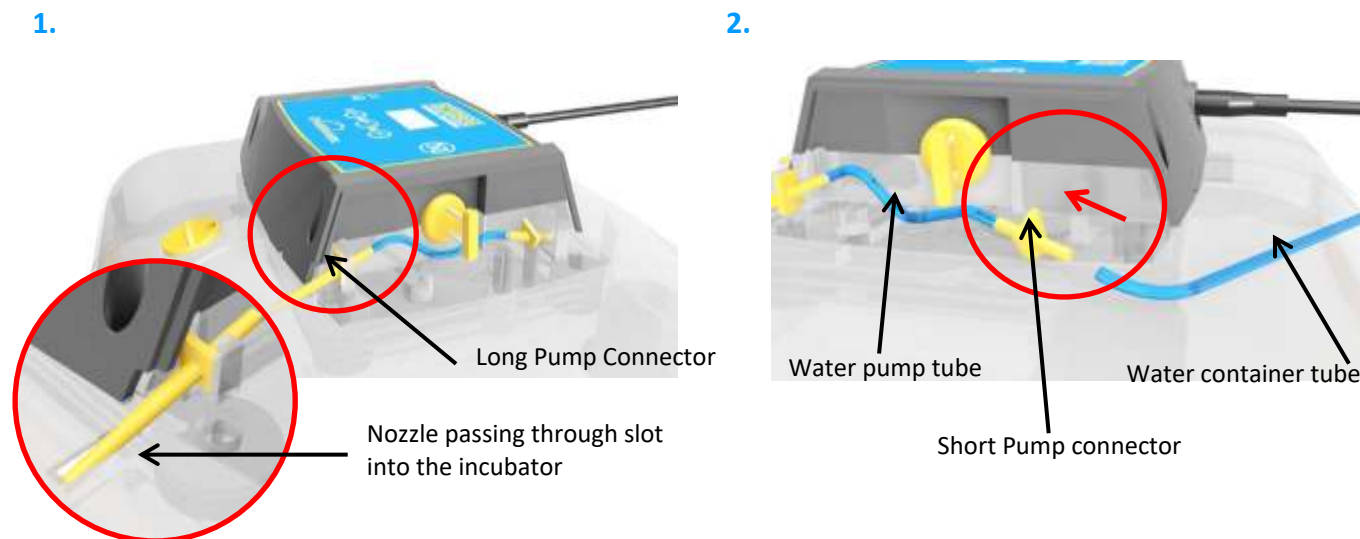
Water Pump Tube diagram to scale
